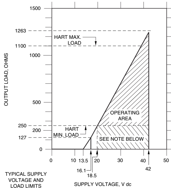
Figure 6. 4 to 20 mA Output, Supply Voltage vs. Output Load
