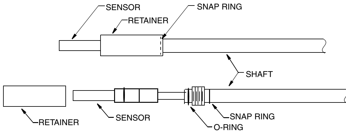
Figure 9. Replacing the Sensor in the Sensor Mounting Type G
