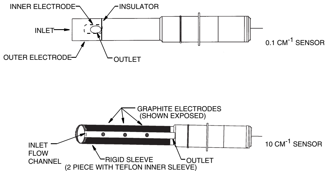
Figure 1. 871CR Sensors
