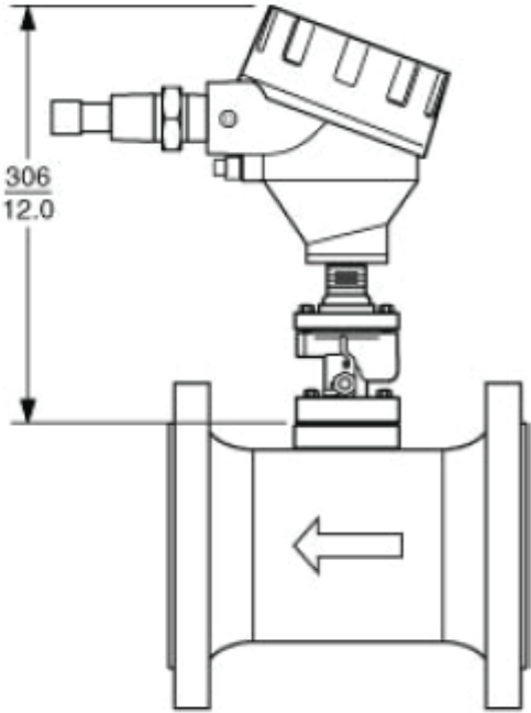
STANDARD TEMPERATURE WITH ISOLATION VALVE
