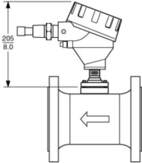
STANDARD TEMPERATURE NO ISOLATION VALVE
