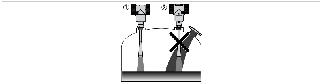
Figure 3-11: Product inlets
