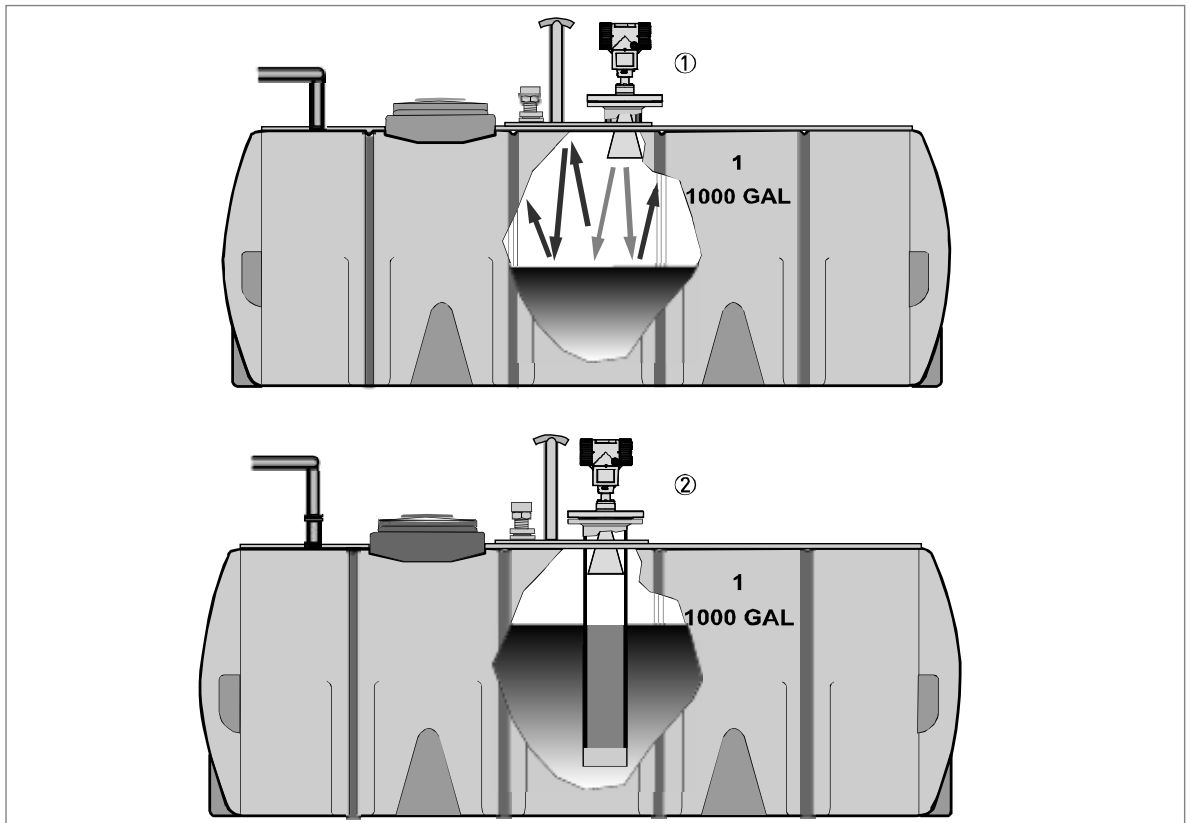
Figure 3-18: Horizontal cylindrical tanks
