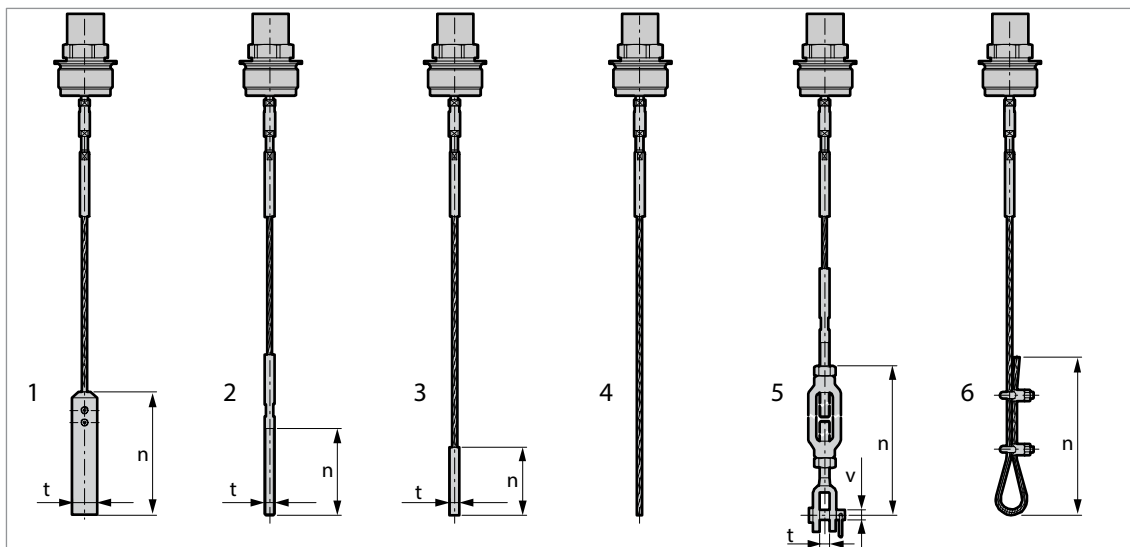
Probe end options for cable probes: single cable Ø4 mm/0.15"
