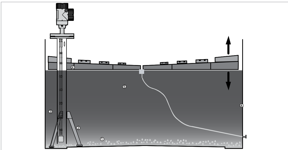
Figure 3-9: Floating roofs
