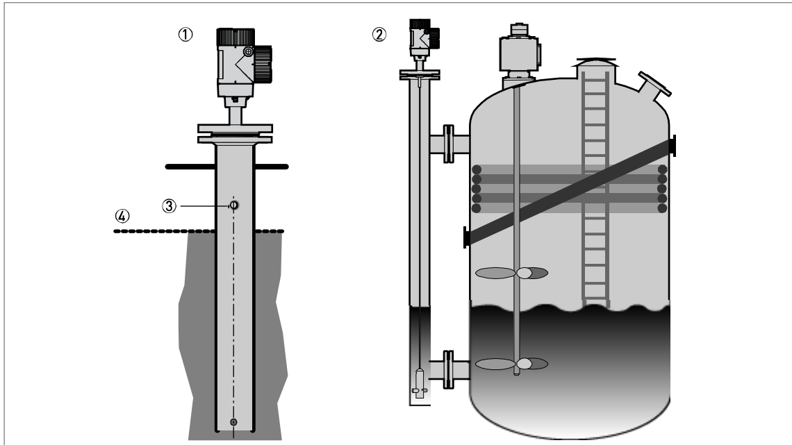
Figure 3-8: Installation recommendations for standpipes (stilling wells and bypass chambers)
